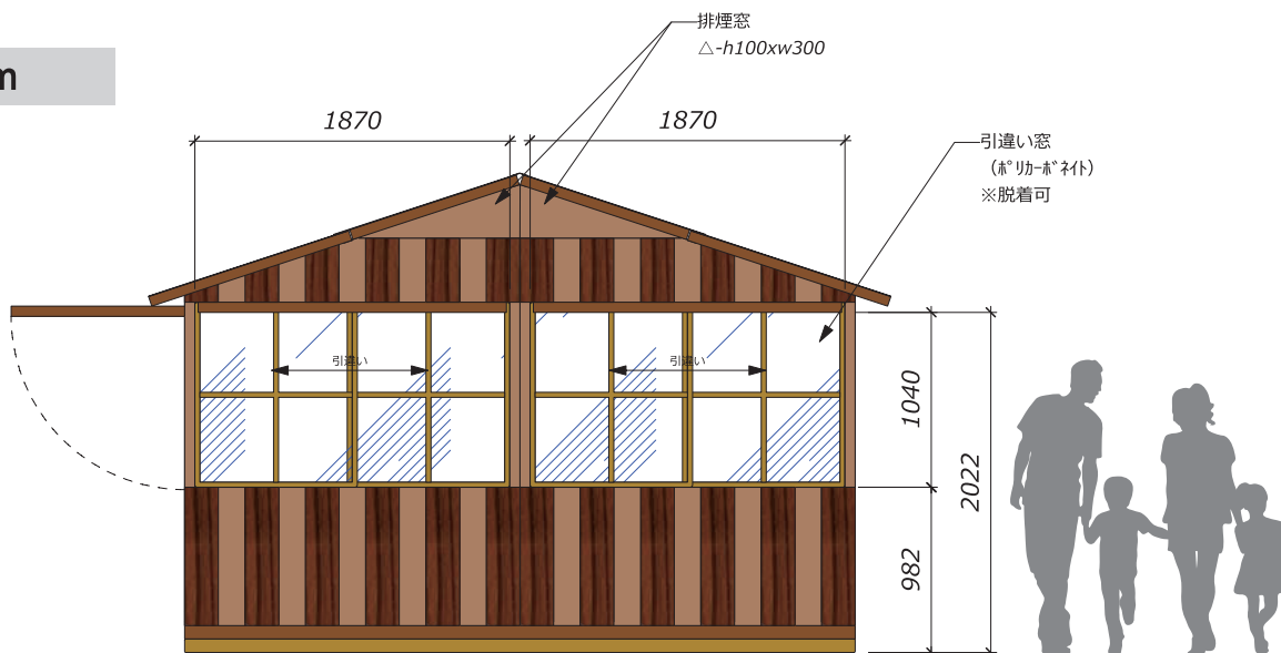
"C" elevation S=1/500
